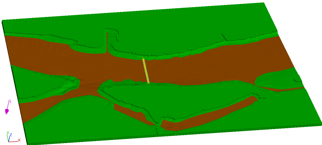
Figure 10 Overview of the Model A geometry. During an ebb (falling tide) flow is from right to left.
