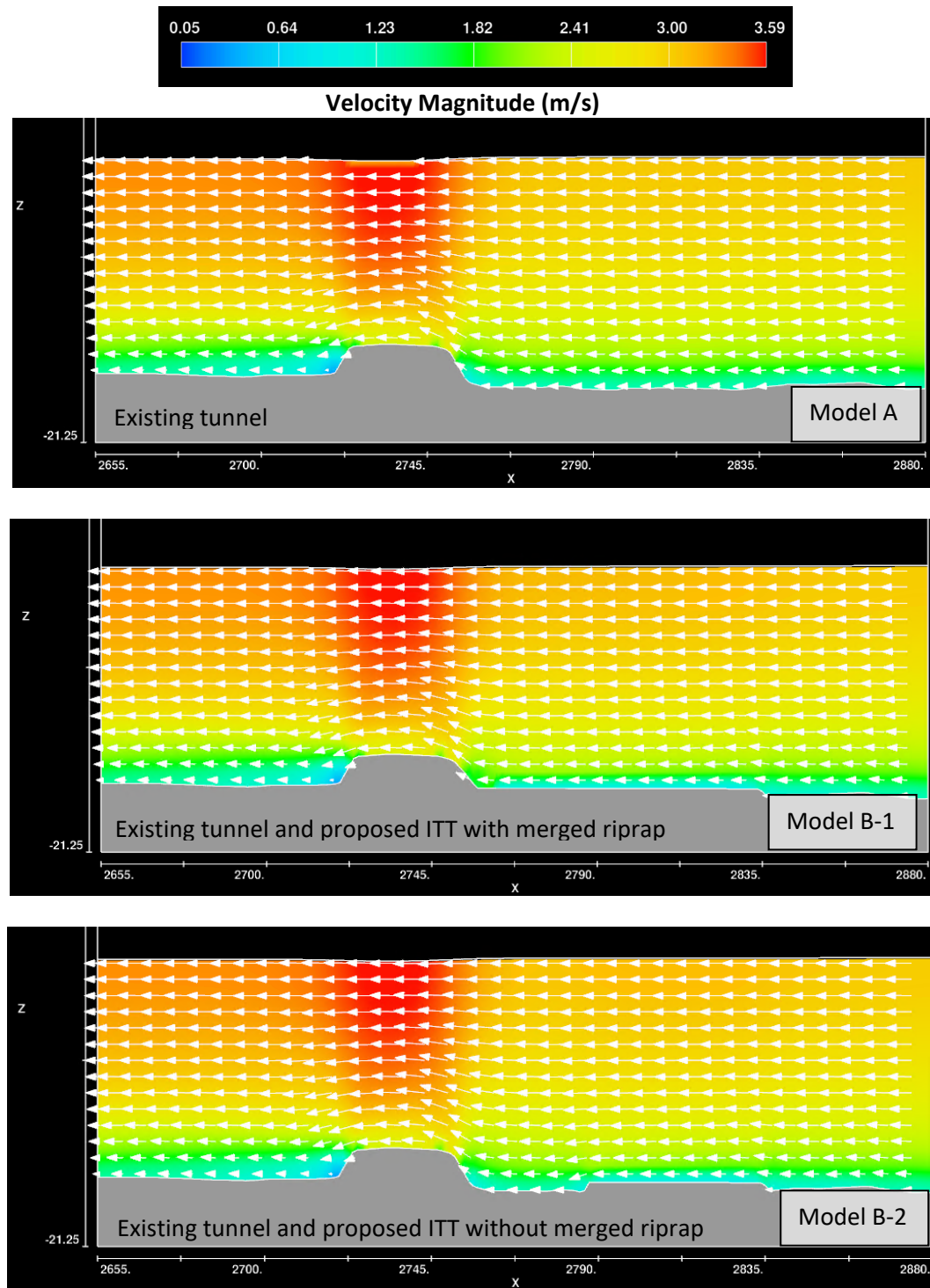
Figure 22 Velocity magnitude (m/s) simulated for the 500-year return period event including moderate climate change and no sea level rise flow condition. Flow is from right to left.
