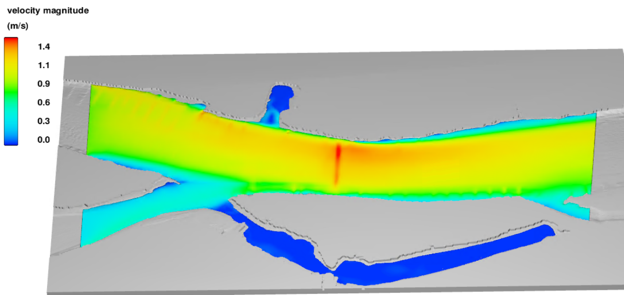
Figure 20 Velocity magnitude simulated in Model A (existing tunnel with bed degradation) for the 2012 King Tide simulation. Flow is from left to right.
