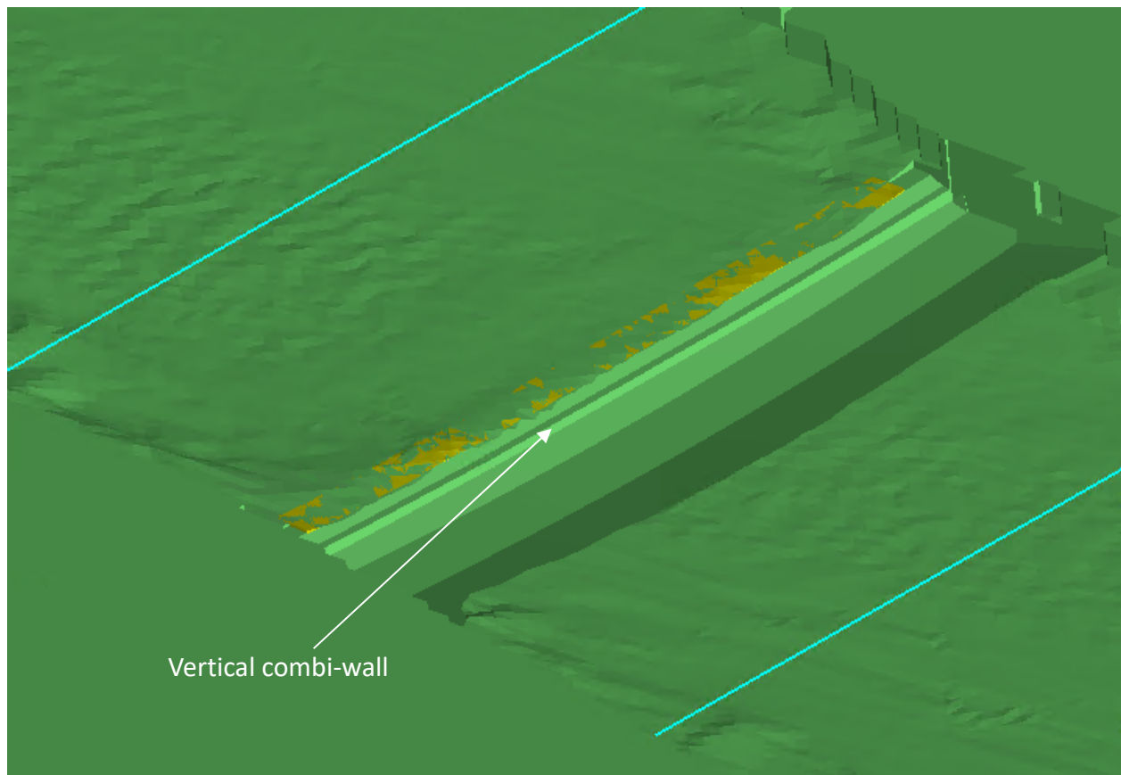
Figure 14 Model C-1: Vertical combi-wall excavation in the model. During an ebb (falling tide) flow is from bottom right to top left.
