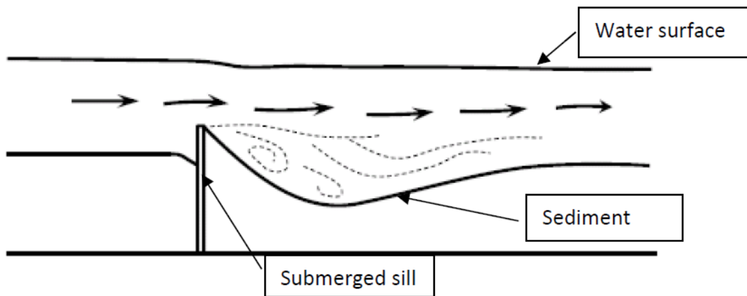
Figure 2 Conceptual diagram of a submerged sill taken from Melville (2014) with annotations added.
