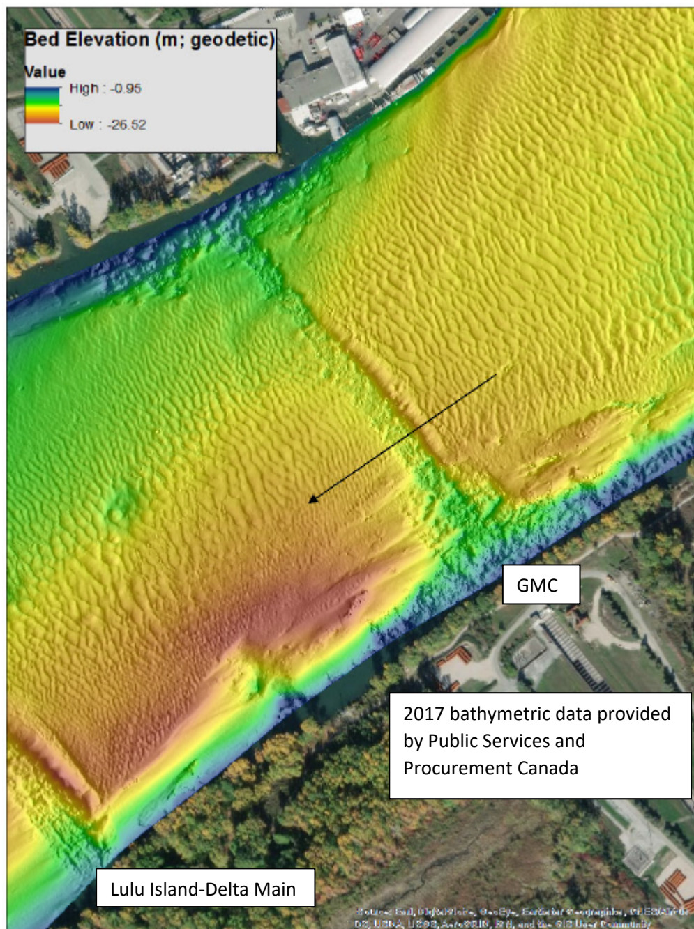
Figure 7 Bathymetry at the George Massey Crossing, collected by Public Services and Procurement Canada in 2017. Black arrow shows location of profile cut presented in Figure 8. During an ebb (falling tide) flow is top right to bottom left.
