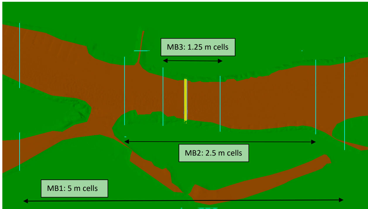
Figure 19 Mesh blocks (MBs) within the GMC CFD model, including the cell size. During an ebb (falling tide) flow is from right to left.
