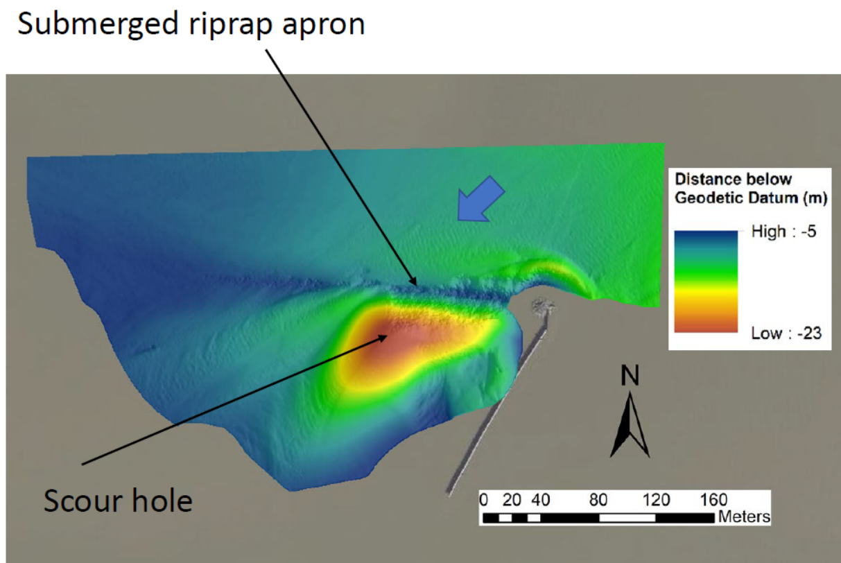
Figure 3 Bathymetric data from Public Services and Procurement Canada at the Trifurcation Wall. During an ebb (falling tide) flow is from top to bottom.
