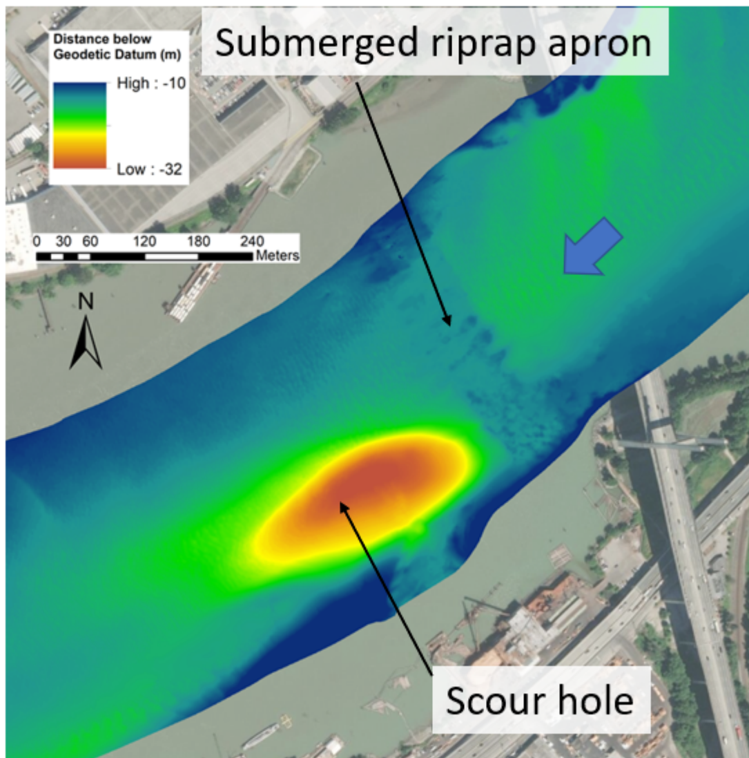
Figure 4 Bathymetric data from Public Services and Procurement Canada at the South Surrey Interceptor. During an ebb (falling tide) flow is from top right to bottom left.
