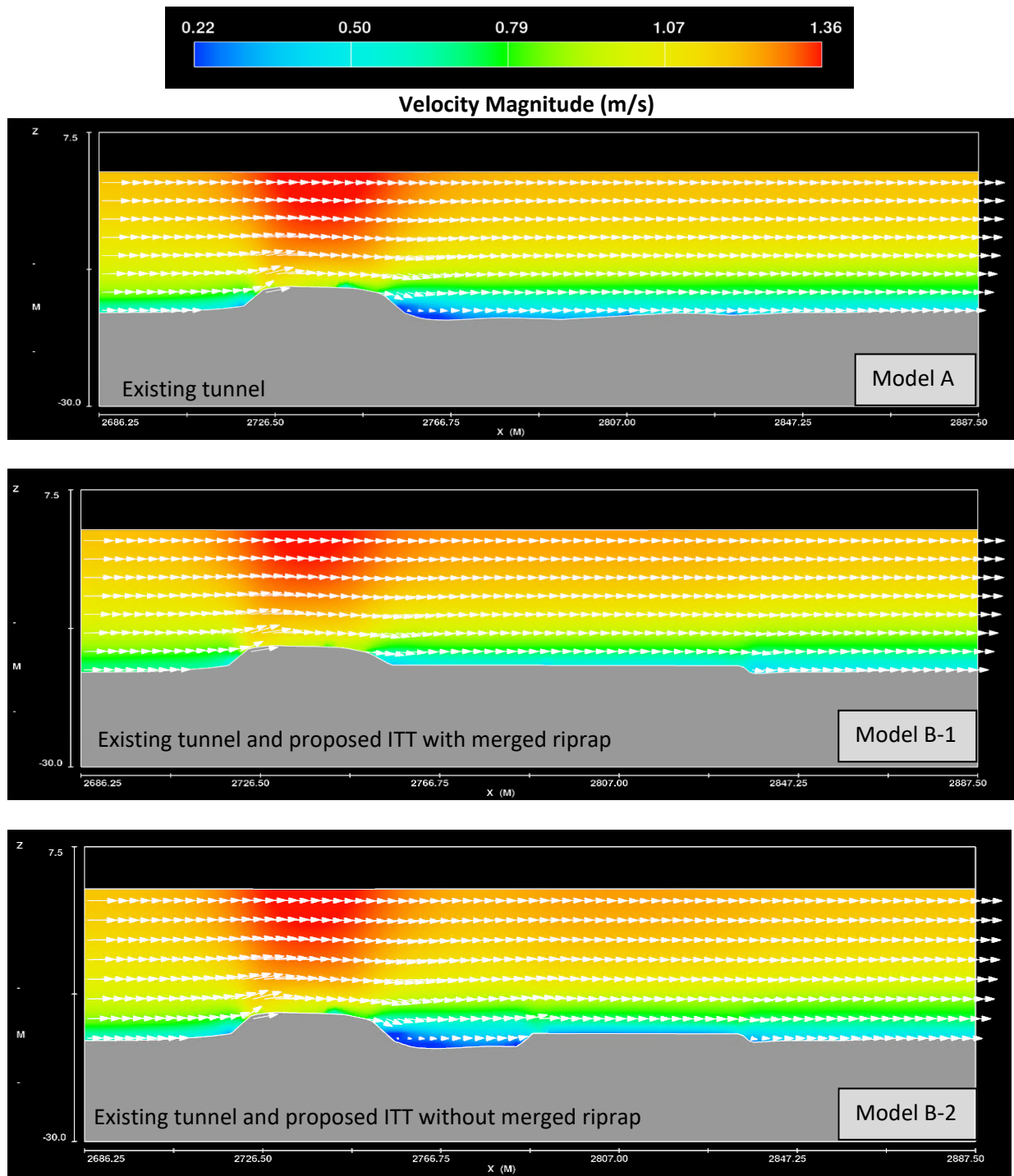
Figure 21 Velocity magnitude (m/s) simulated for the 2012 King Tide flow condition. Flow is from left to right.
