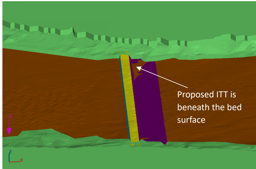
Figure 17 Model B-1 geometry: Existing tunnel and proposed ITT (with merged riprap). During an ebb (falling tide) flow is from right to left.
