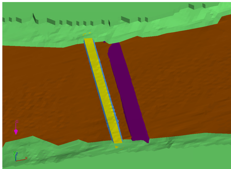
Figure 18 Model B-2 geometry: Existing tunnel and proposed ITT (without merged riprap). During an ebb (falling tide) flow is from right to left.
