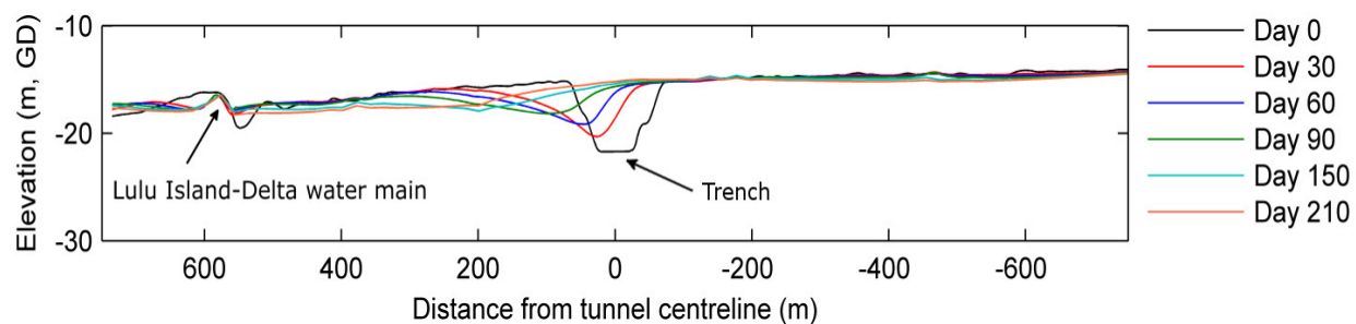
Figure 27 Downstream trench migration, predicted by NHC's (2015b) numerical model, following the removal of the existing GMC. During an ebb (falling tide) flow is from right to left.
