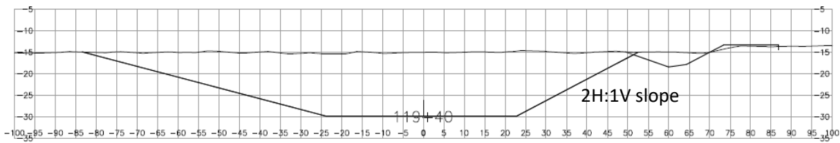
Figure 15 Drawing of 2H:1V sloping excavation provided by Stantec (received by NHC on September 3, 2019). During an ebb (falling tide) flow is from left to right.
