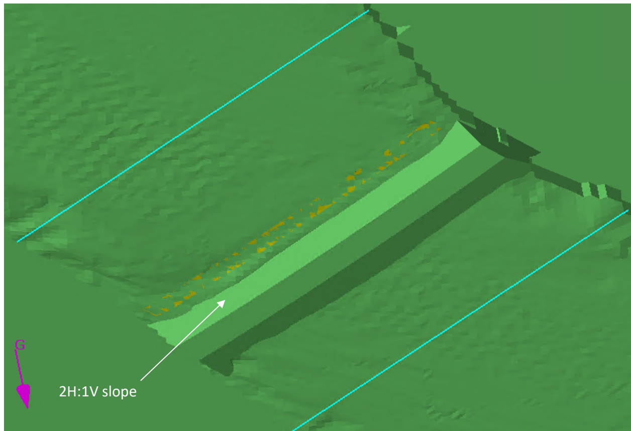
Figure 16 Model C-2: 2H:1V sloping excavation in the model. During an ebb (falling tide) flow is from bottom right to top left
