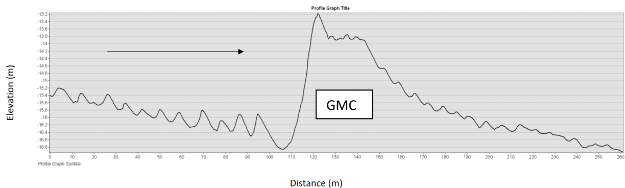
Figure 8 Bathymetric profile over the existing George Massey Crossing. Location of cut is shown in Figure 7. During an ebb (falling tide) flow is from left to right.
