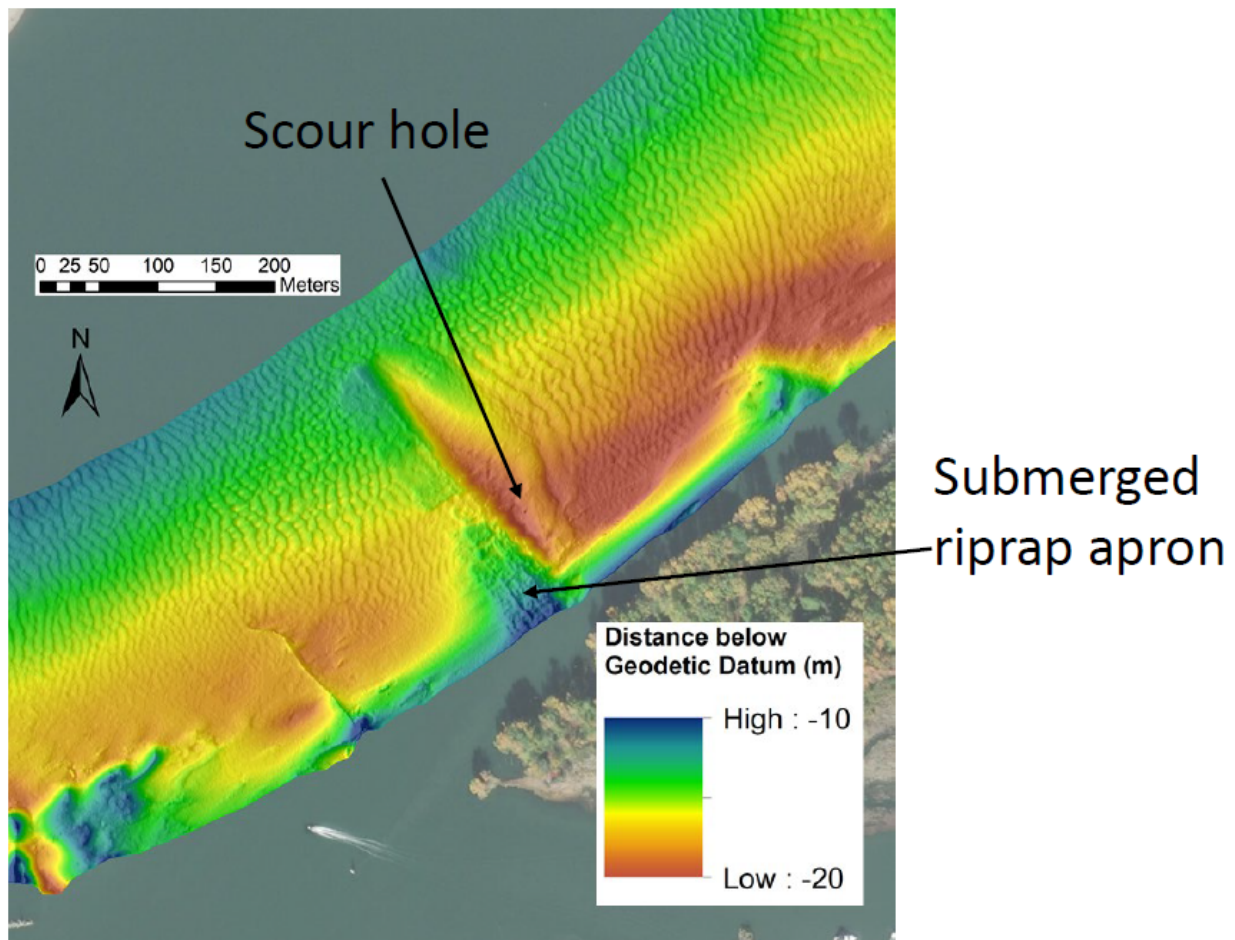
Figure 5 Bathymetric data from Public Services and Procurement Canada at the Lulu Island-Delta Water Main. During an ebb (falling tide) flow is from top right to bottom left.
