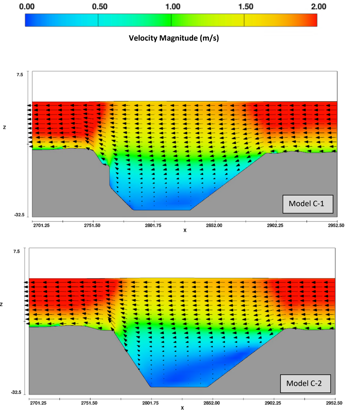
Figure 26 Longitudinal profile in vertical plane – Velocity magnitude (m/s) simulated during the 2012 August Flow Simulations in Models C-1 and C-2. Flow is from right to left.
