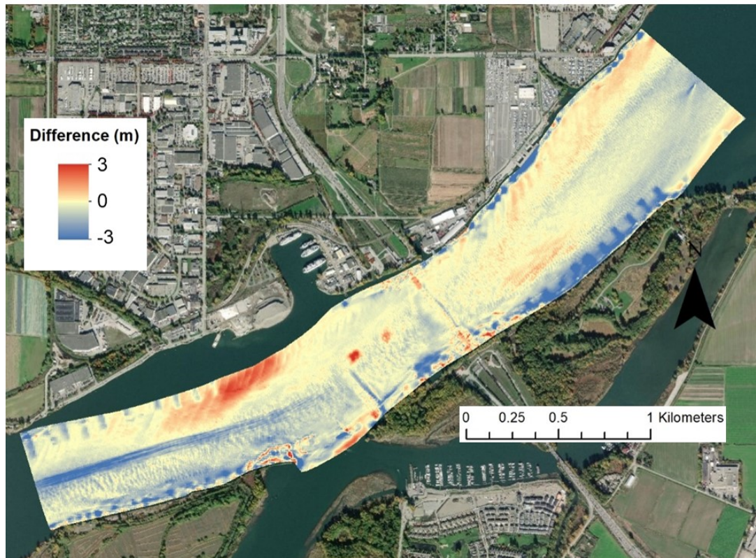
Figure 12 Difference in bed elevation between 2017 (data collected by PSPC, formerly PWGSC) and 2004 (data collected by PWGSC). During an ebb (falling tide) flow is from top right to bottom left.
