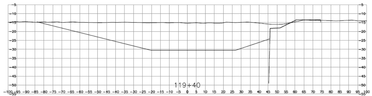
Figure 13 Drawing of vertical combi-wall excavation provided by Stantec (received by NHC on August 29, 2019). During an ebb (falling tide) flow is from left to right.
